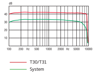
FREQUENCY RESPONSE
